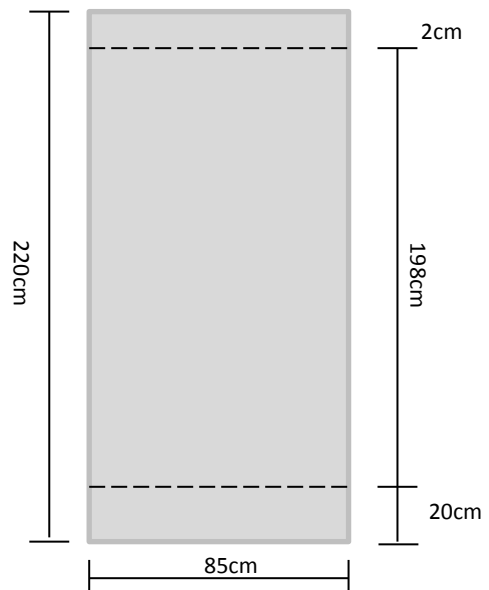
Pole can be stored in the base of the Roll Up
